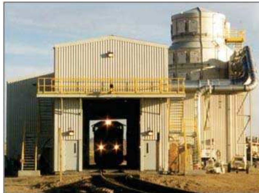
Figure 1. Bottom dump station with dust collection unit. Courtesy of: Aircure
